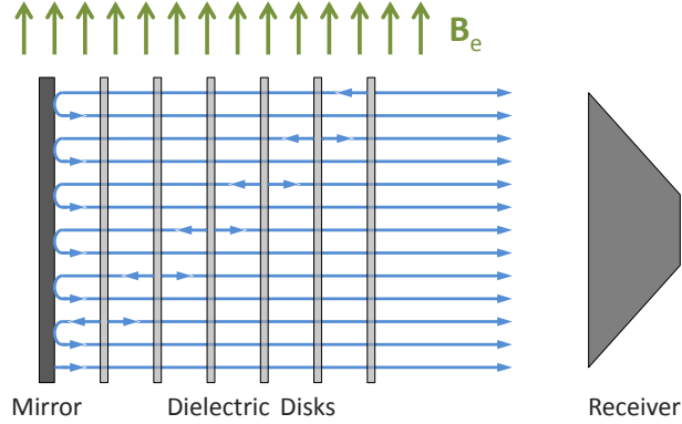
Figure 4. A dielectric haloscope consisting of a mirror and several dielectric disks placed in an external magnetic field \mathbf{B}_e and a receiver in the field-free region. A focusing mirror (not shown) could be used to concentrate the emitted power into the receiver. Internal reflections are not shown. Figure taken with permission from [30].
