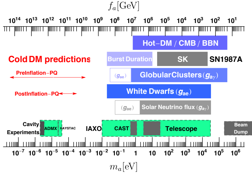
Figure 1. Overview of axion masses m_a (equivalently f_a ) excluded by a variety of astrophysical and cosmological arguments (blue) or laboratory searches (gray) together with experimental prospects (green) and axion cold DM predictions. Pre- and postinflation PQ breaking scenarios are explained in section 2.4.
