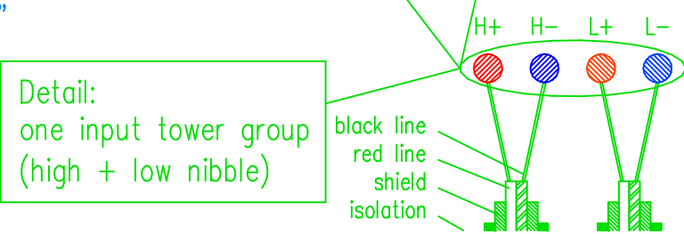
input for daughterboard type "B"
